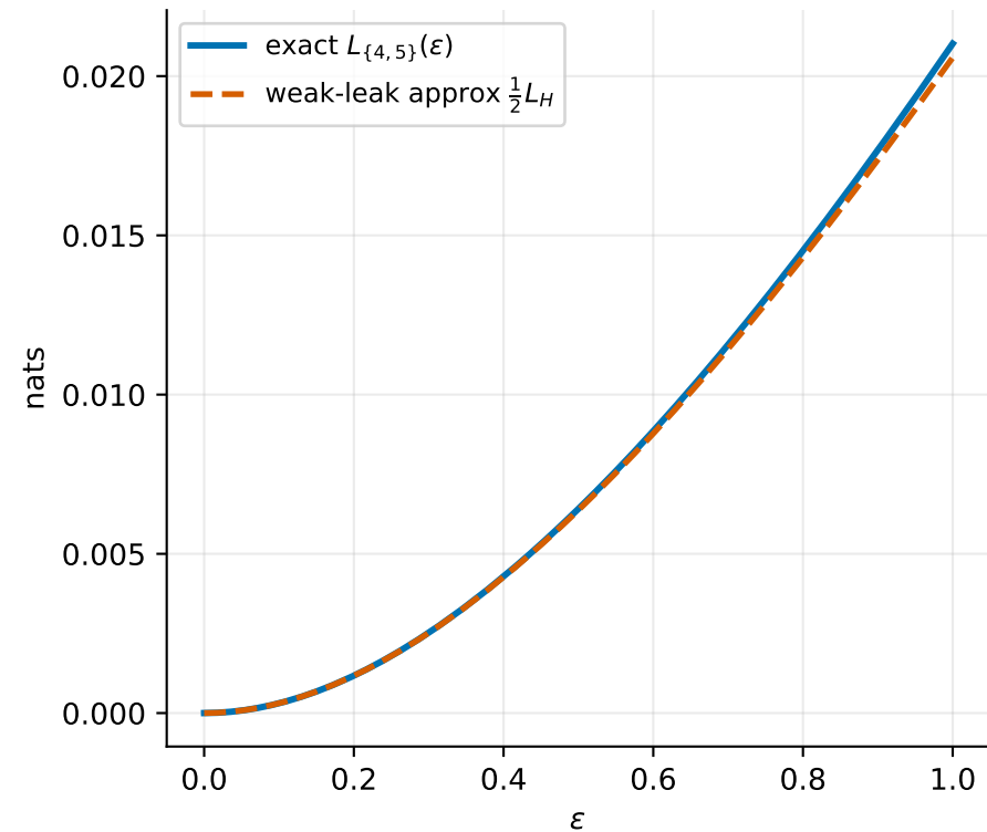
A: exact CMI vs. Hessian (weak-leak) approximation
