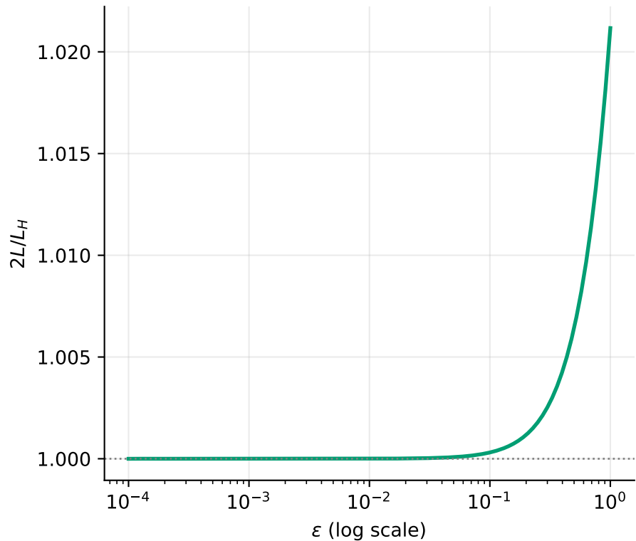
B: departure of 2L/L_H from unity
