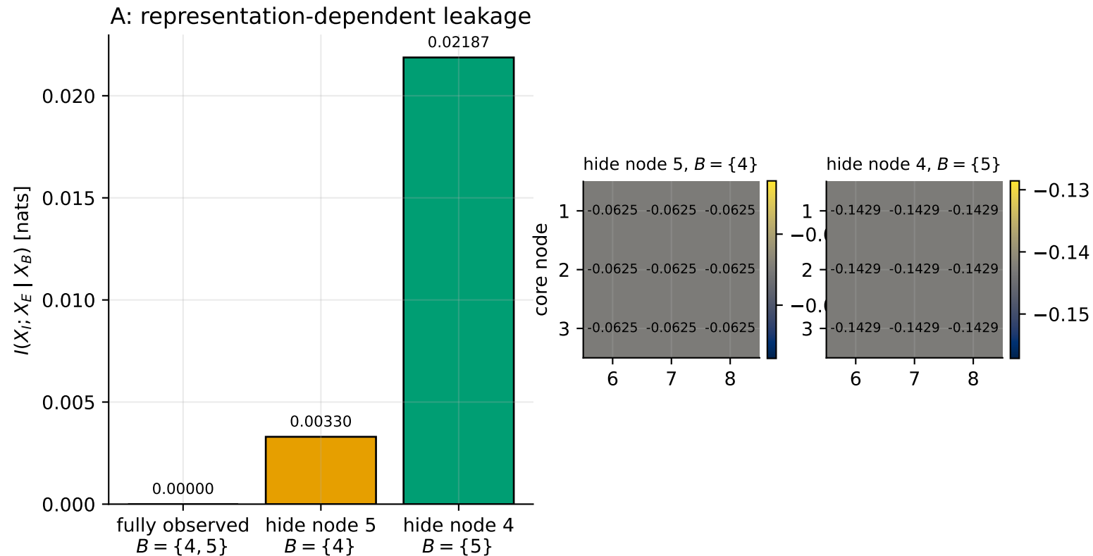
Figure 4 — Observer/representation dependence of the inferred blanket
