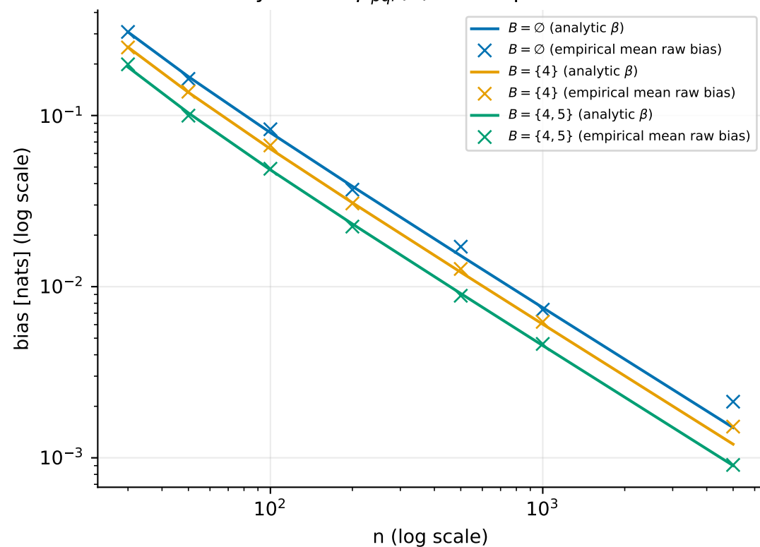
C: analytic bias \beta_{pqr}(n) vs. empirical raw bias
