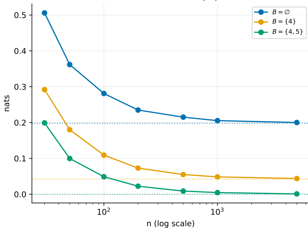
C: analytic bias \beta_{pqr}(n) vs. empirical raw bias
