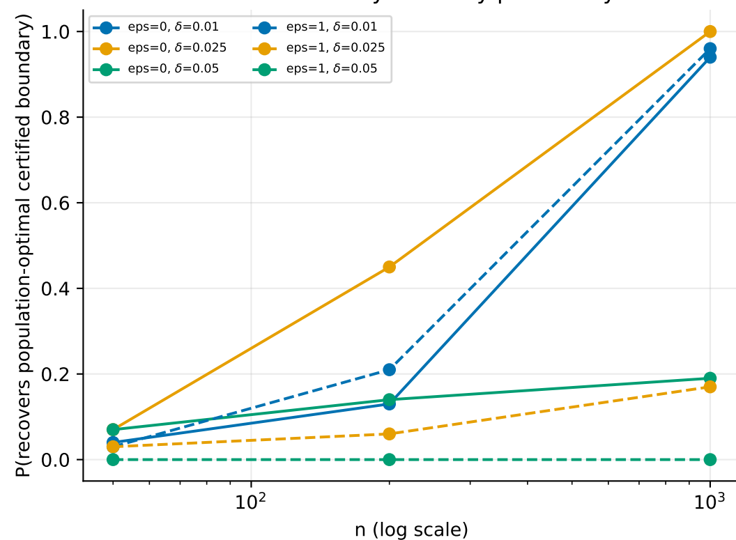
D: certified-boundary recovery probability vs. n
