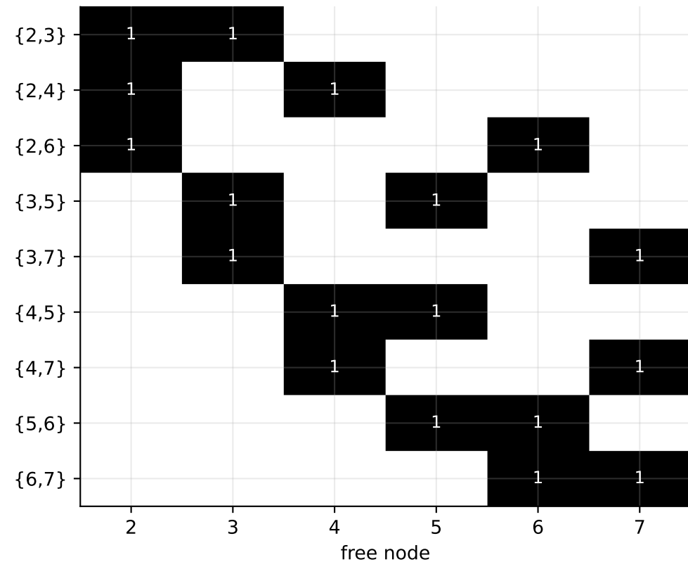
A: the 9 exact minimum separators (anchored 1 \in I , 8 \in E , |B| = 2 )
