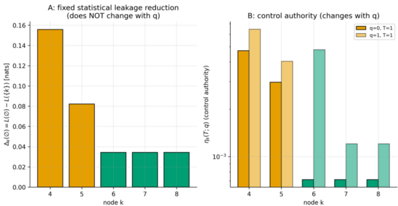
Steering Figure 8 — Statistical boundary vs. control interface
