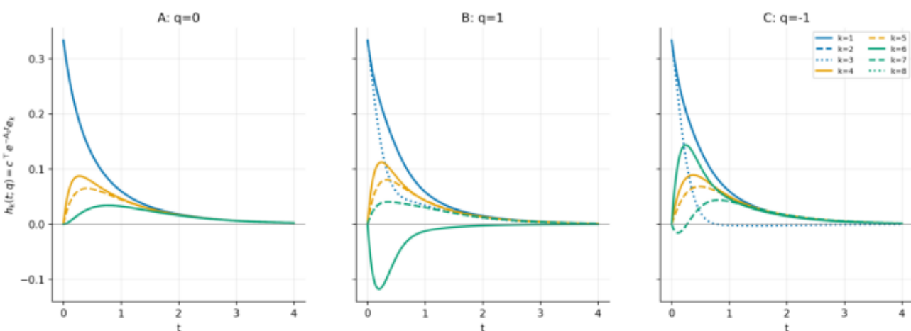
SFig 3: Impulse-response atlas Steering Figure 3 — Impulse-response atlas
