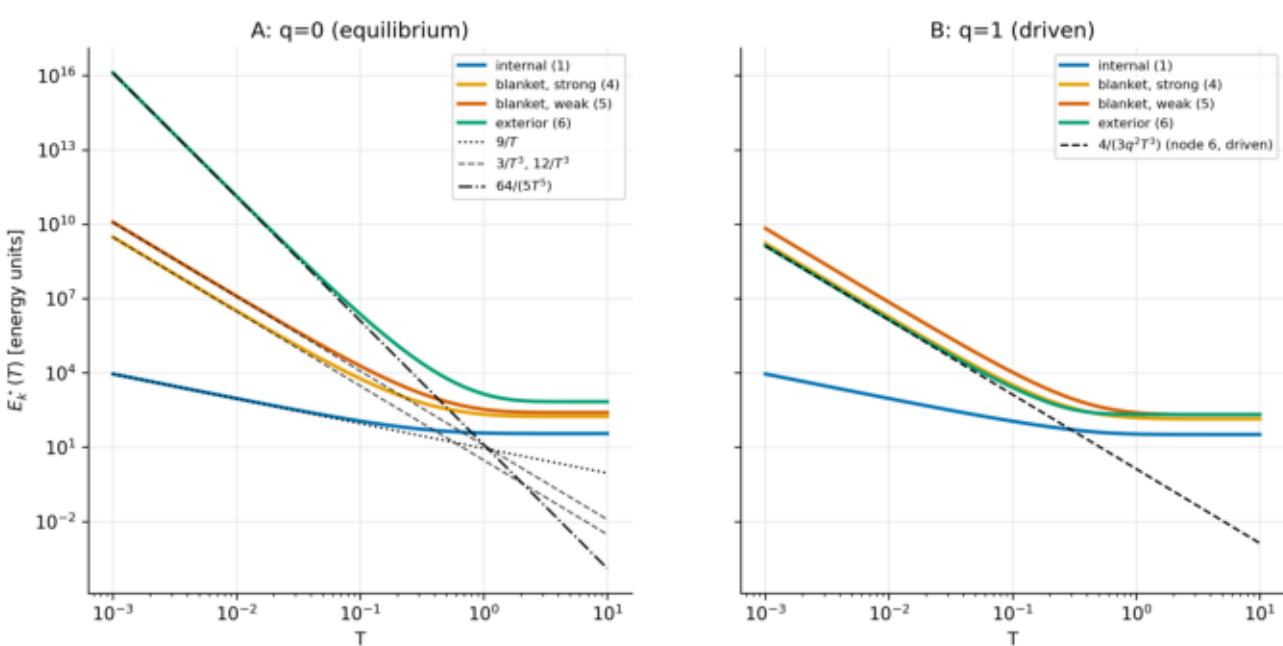
Steering Figure 5 — Minimum energy vs. time horizon
