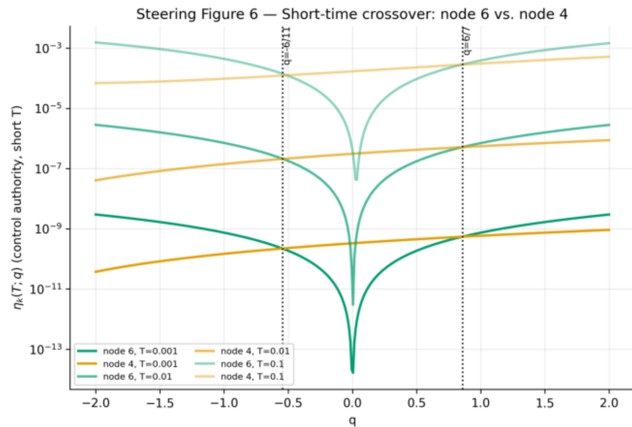
SFig 6: Short-time crossover
