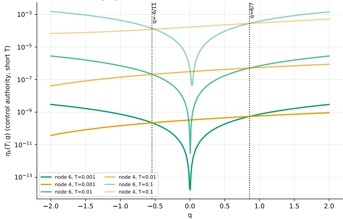
Steering Figure 6 — Short-time crossover: node 6 vs. node 4
