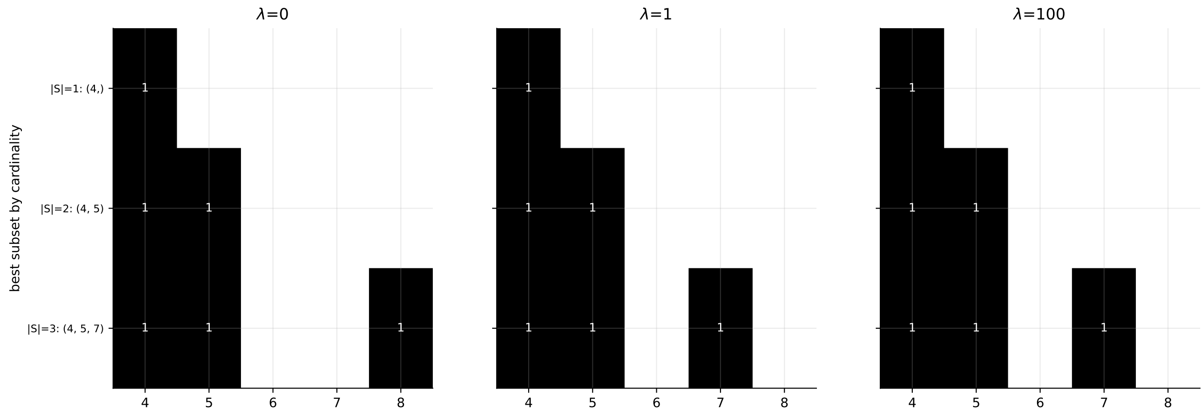
Stage-4 Figure 10 — Composition of best sparse actuator sets ( q=0 , T=1 )
