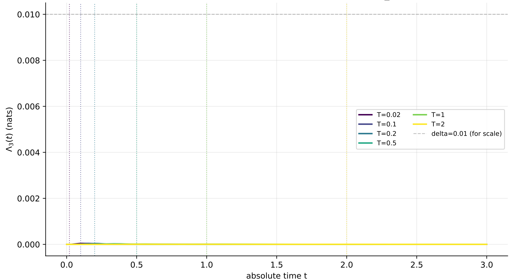
Audit Fig A: existing [0, T_{\text{ramp}}] window (dotted lines) vs full relaxation (the old Fig-3 right panel only ever looked at t \leq T_{\text{ramp}} )
