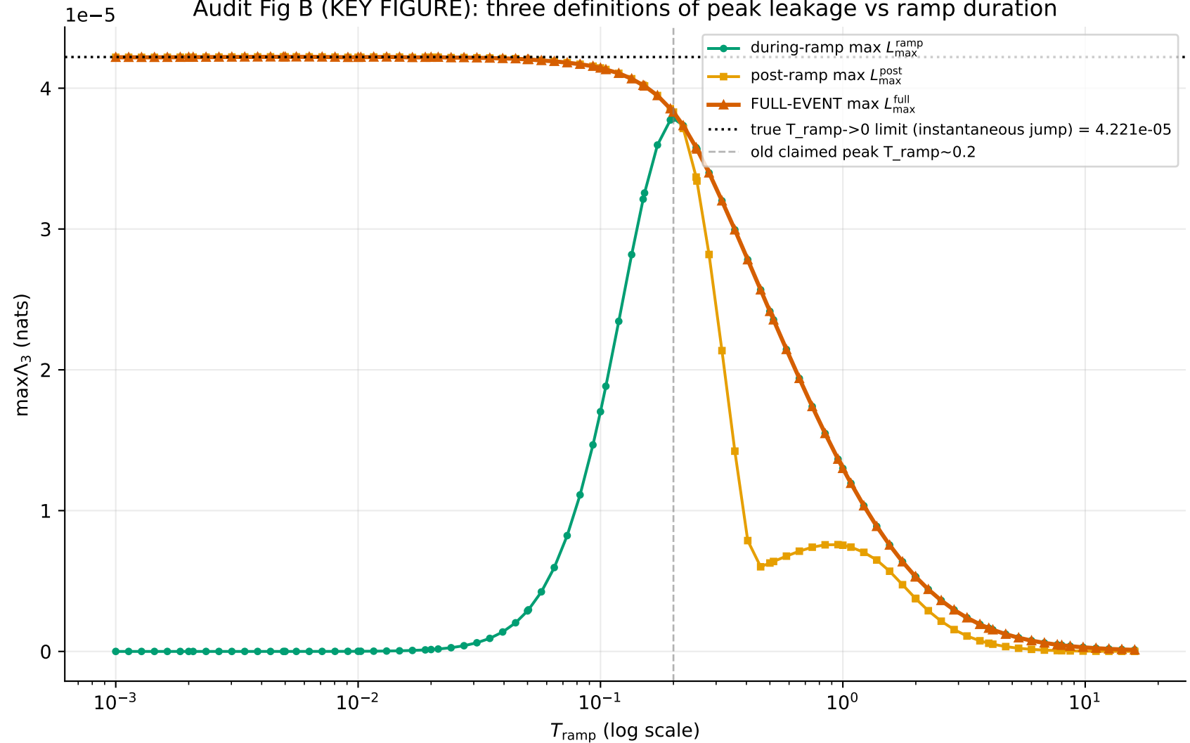
Audit Fig B (KEY FIGURE): three definitions of peak leakage vs ramp duration
