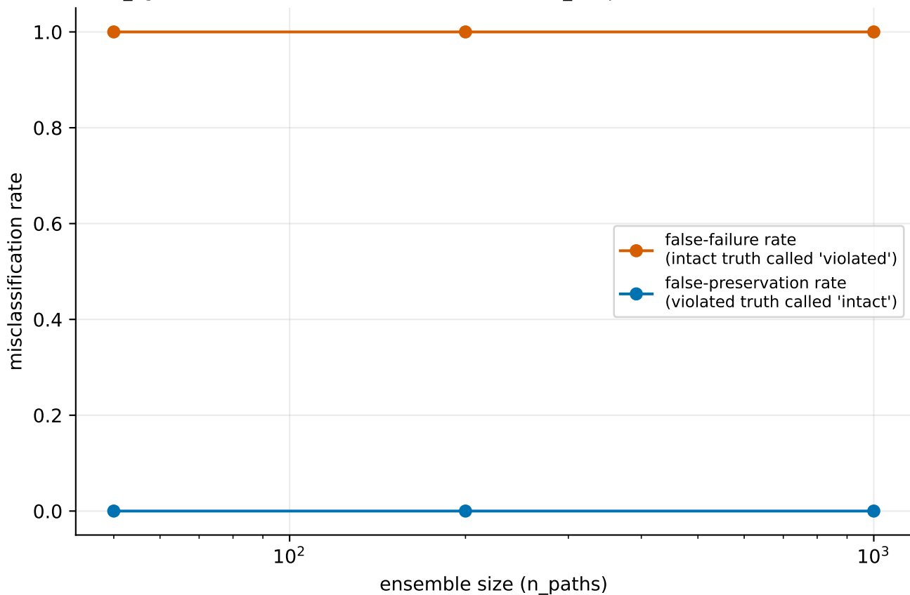
Simultaneous-band pathwise classification error vs. sample size (delta_fig11=1e-05, 40 realizations/cell, true classes: T_ramp in [0.1, 0.15, 0.2, 0.25] vs [4, 8])
