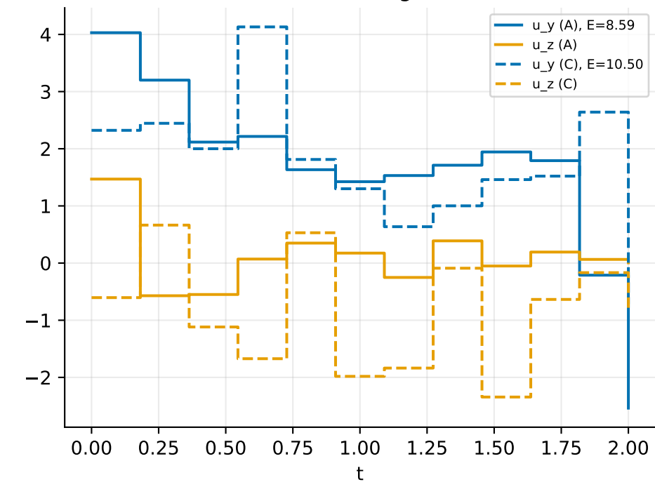
Panel C: controls (energies annotated)
