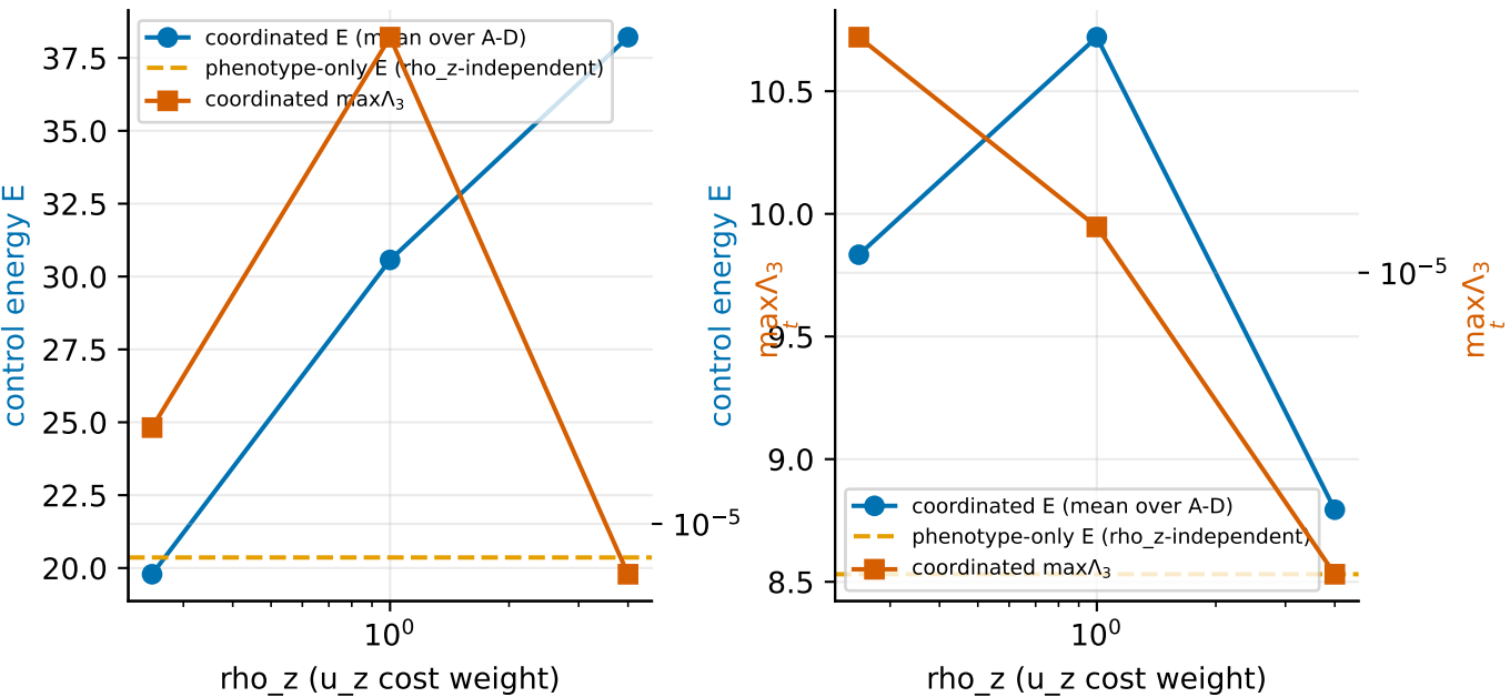
Row 2: \rho_z sensitivity (coordinated control only; formulations A-D averaged)
