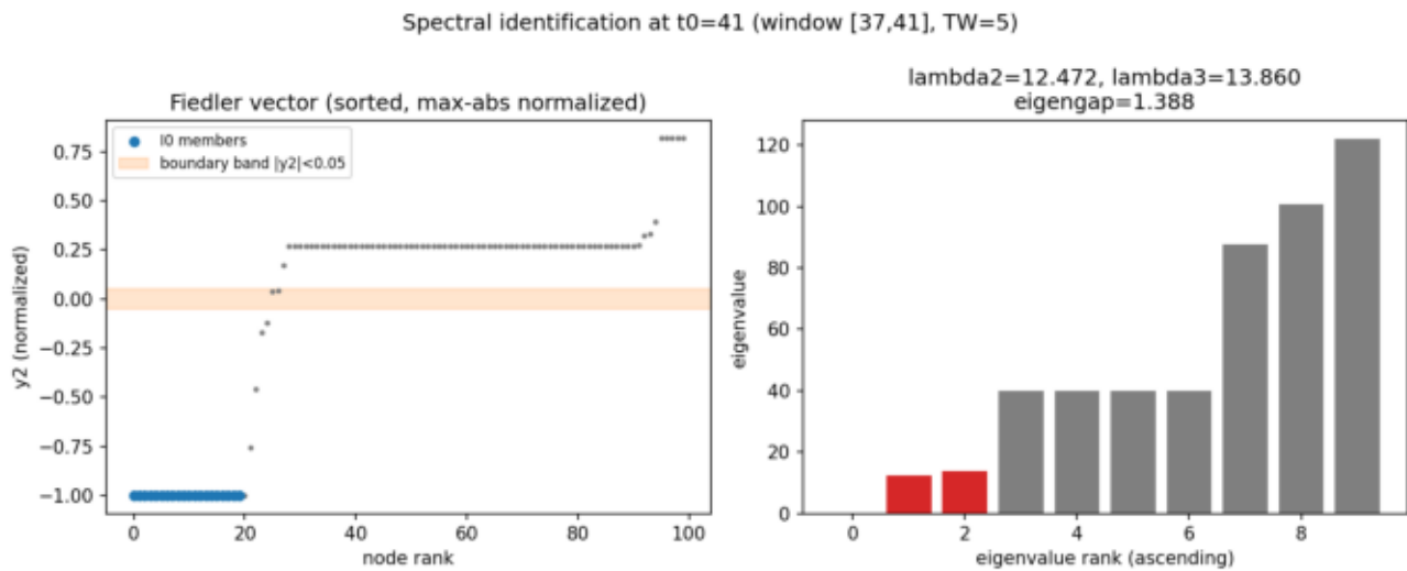
fig02_spectral_identification.png
