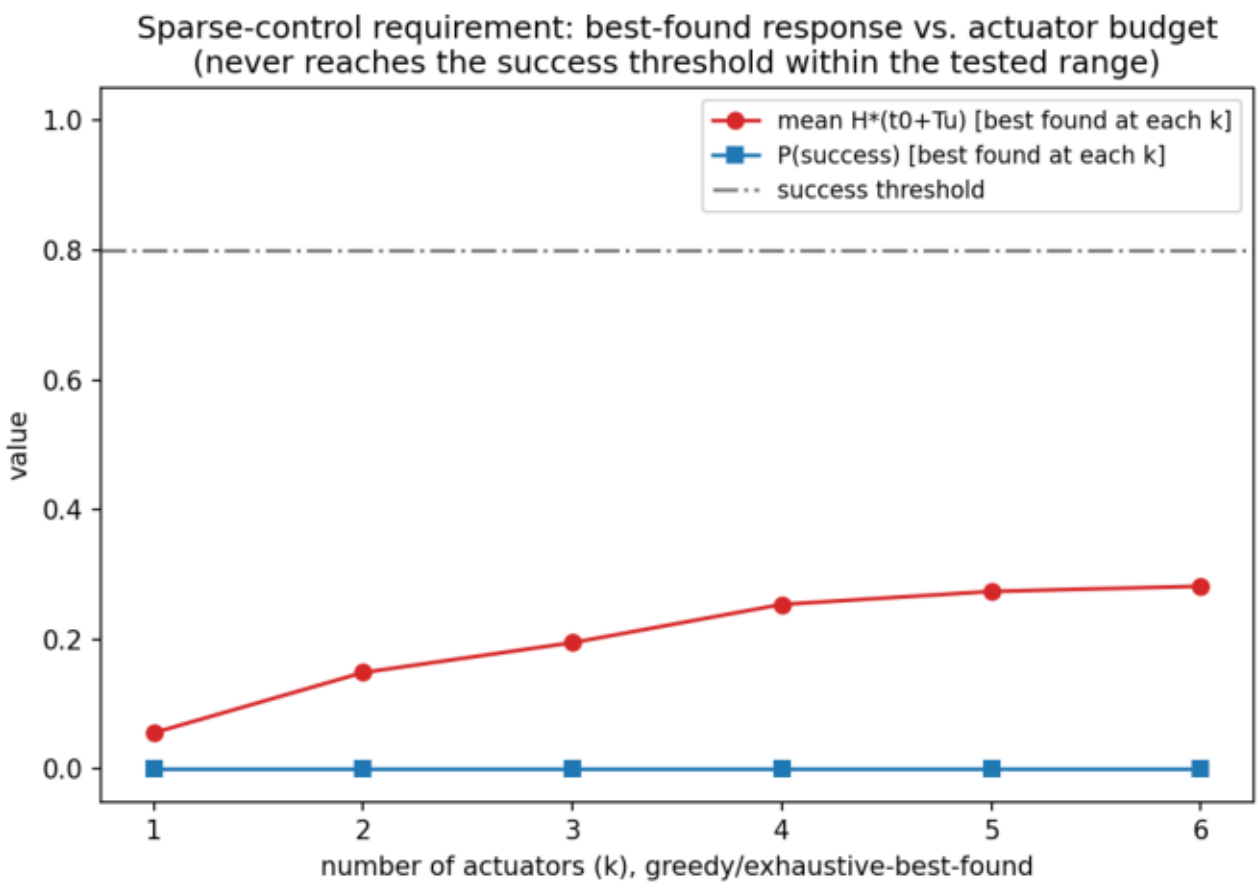
fig07_sparse_requirement.png
