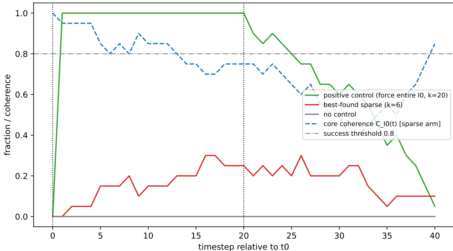
Steering trajectory (single representative replicate, seed=100000) control window: [0, t_u] ; dotted vertical lines mark control on/off
