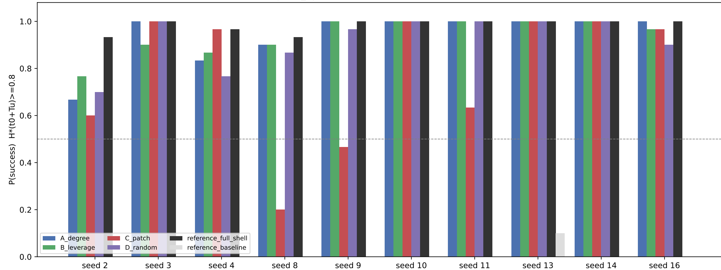
V2 replication: P(success) by rule, across 10 independently emergent flocks ( k = \text{ceil}(0.75 \times |B^D_0|) ), frozen from the canonical-flock mechanism audit)
