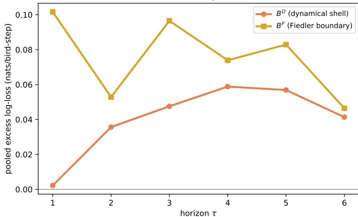
B^D : exact at \tau=1 , grows with horizon (E \rightarrow B \rightarrow I propagation). B^F leaks MORE at every horizon tested.
