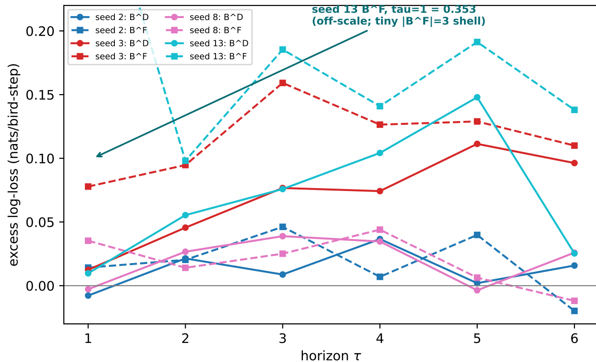
per-flock predictive leakage vs. horizon (solid= B^D , dashed= B^F )
