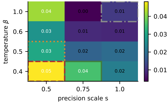
susceptibility \chi
