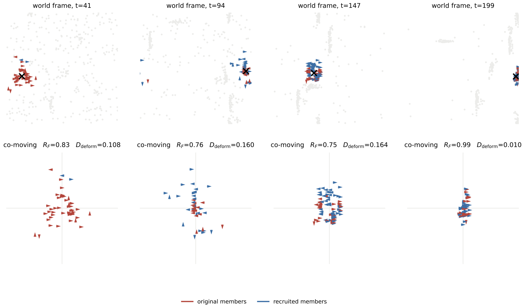
Fig. 6.9-4 The same collective in world coordinates (top) and after subtracting its ESTIMATED translation (bottom). The world-frame group crosses the torus; the co-moving representation stays in place while its membership turns over.
