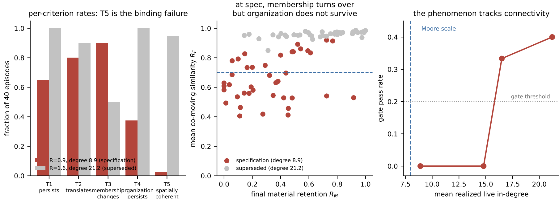
Fig. 6.9-G The feasibility gate FAILS at the specified interaction scale (0/40). Membership turnover is plentiful ( T3 = 0.90 ) but the group fragments into \sim 3.8 pieces and its co-moving organization does not persist ( T4 = 0.38 ). The phenomenon appears only at \sim 3\times Moore connectivity.
