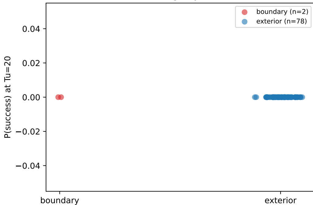
Control leverage by Fiedler role
