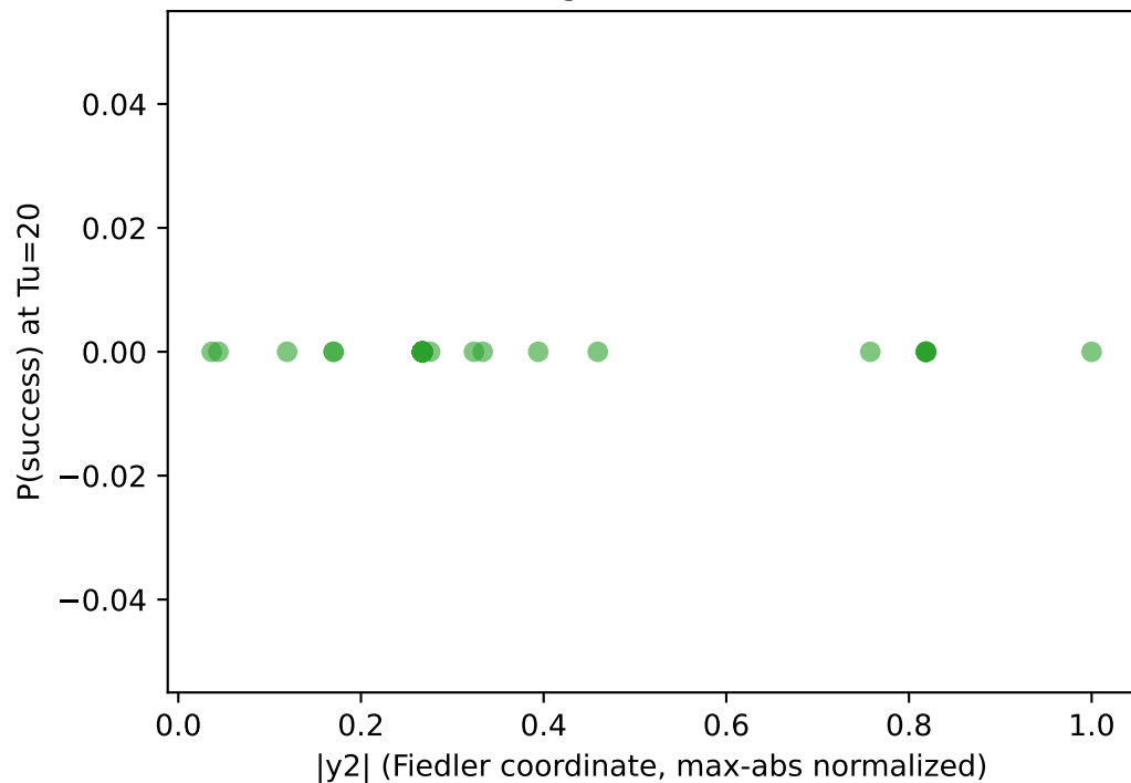
Control leverage vs. Fiedler coordinate
