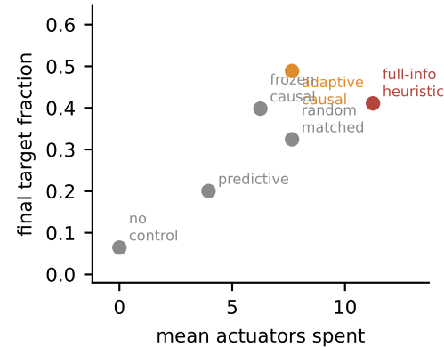
H1 spend does not buy the outcome
