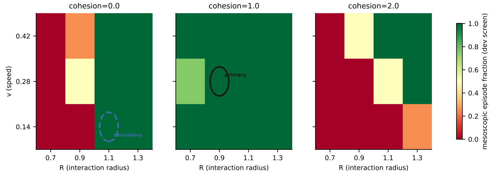
Fig 6.11-1 Phase map: disorder / mesoscopic / global-collapse regimes (global-collapse probability = 0.00 in every cell)
