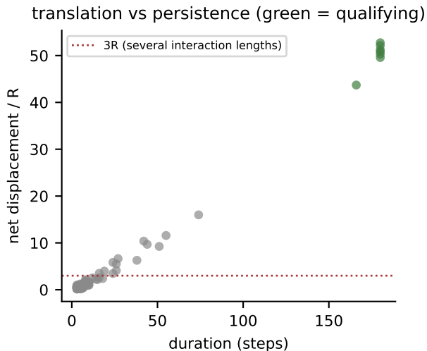
Fig 6.11-2 Spontaneous emergence: domain persistence and translation (primary regime, held-out episode)
