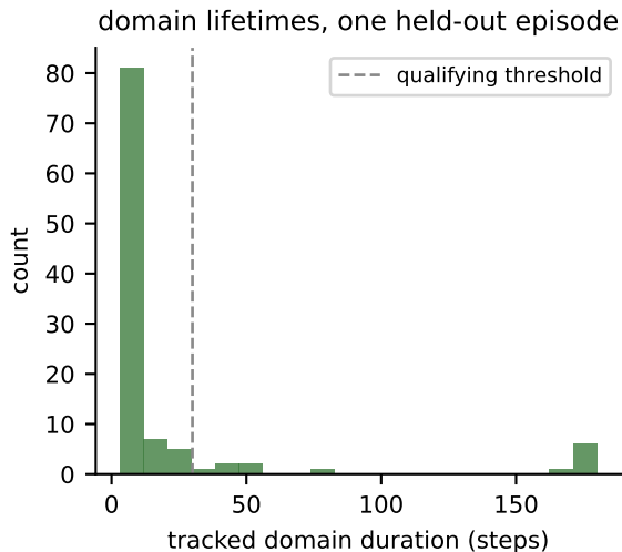
Fig 6.11-2 Spontaneous emergence: domain persistence and translation (primary regime, held-out episode)
