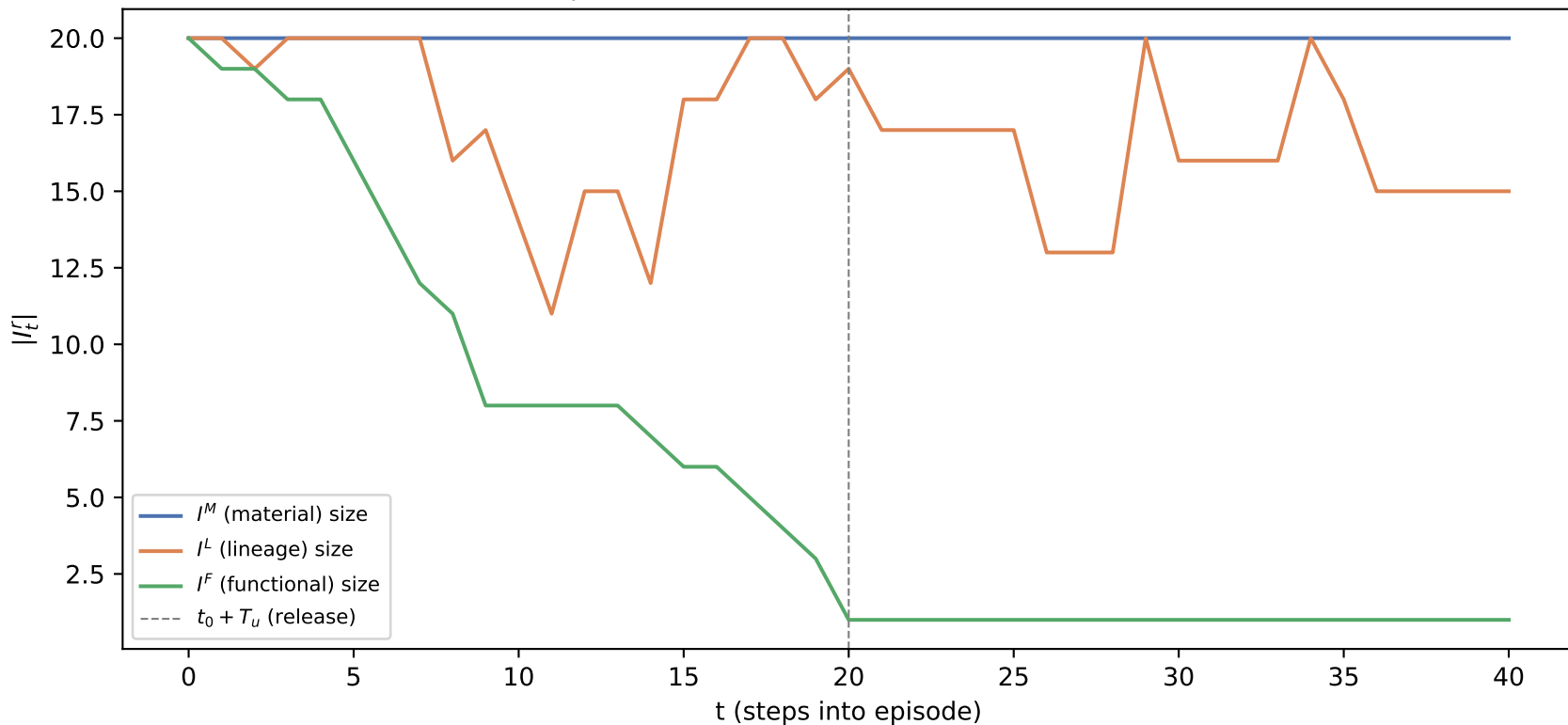
Flock 2, replicate 0: collective size under three definitions
