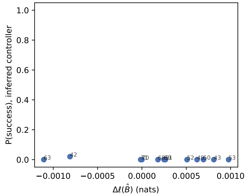
R6.5-3 (exploratory): inference quality vs. control success, 12 discriminating flocks
