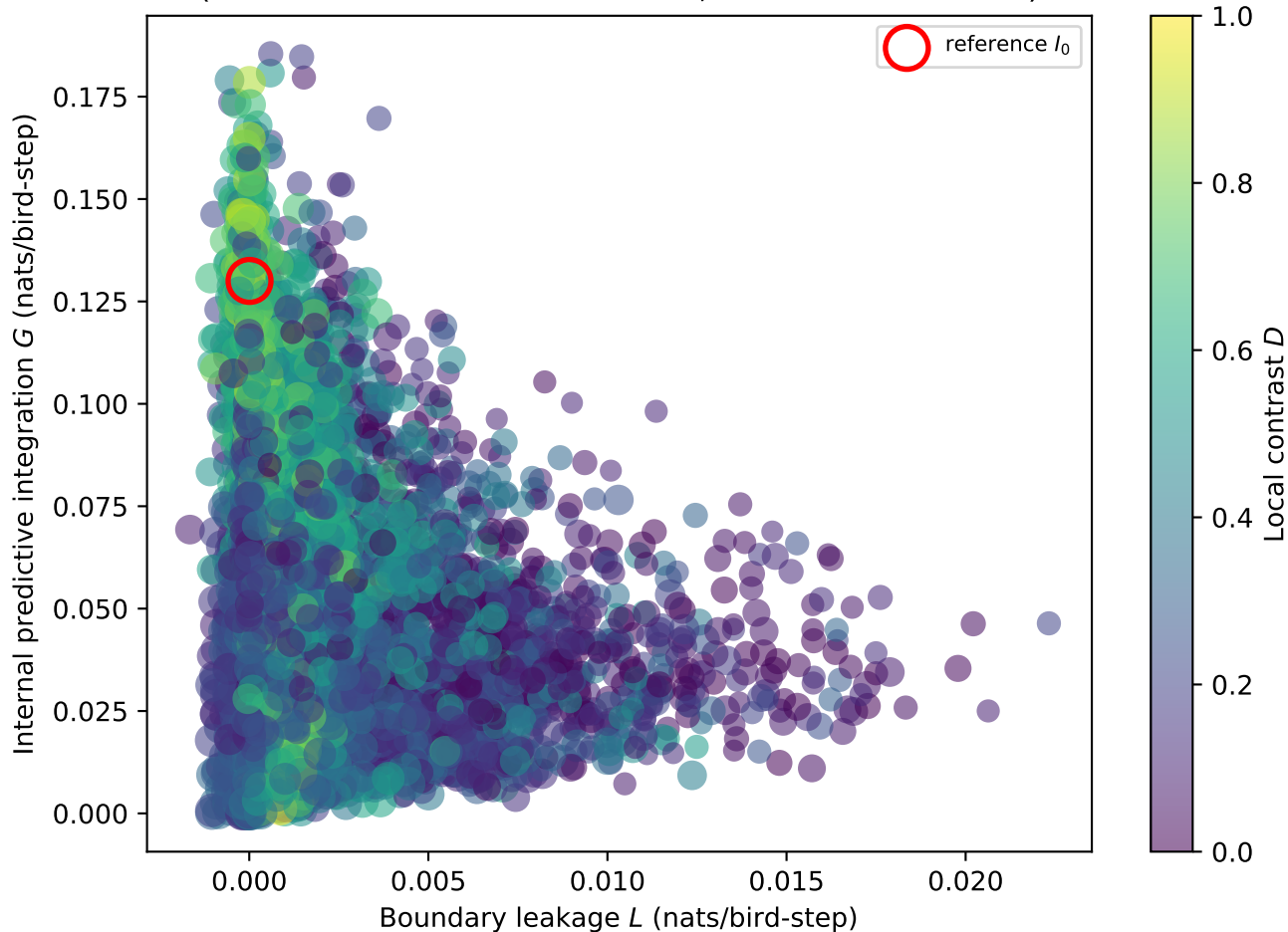
Figure 6.6-1: Collective landscape, seed 4, no_control (5000 candidate k=20 interiors; size = coherence C)
