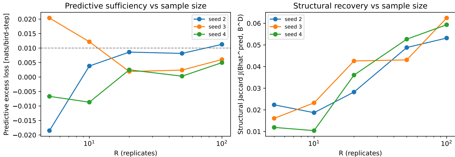
Fig. 6.7-4: sample-efficiency sweep
