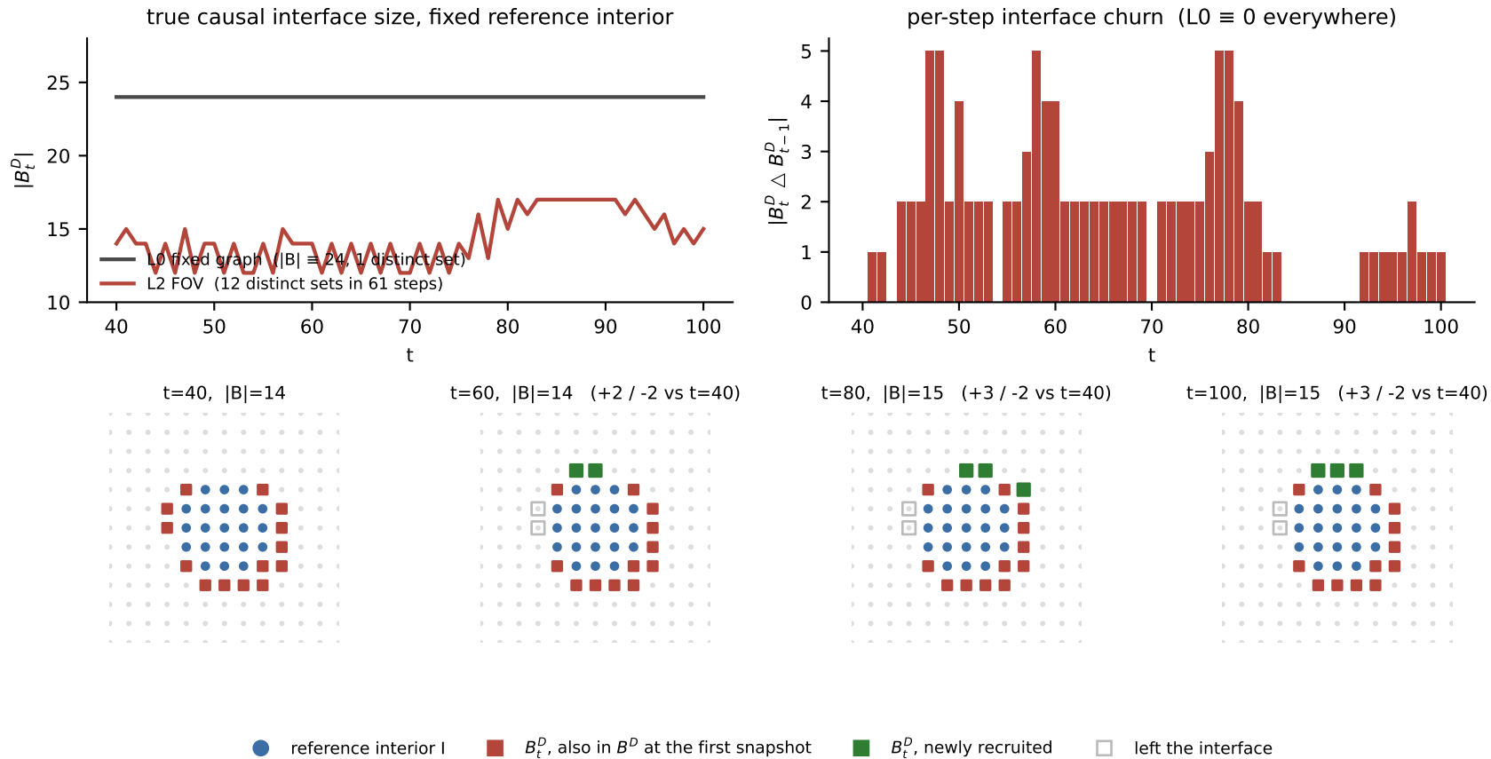
Fig. 6.8-2 The true FOV causal interface changes as birds reorient (seed 70). The interior is held fixed, so every change is the interface's own.
