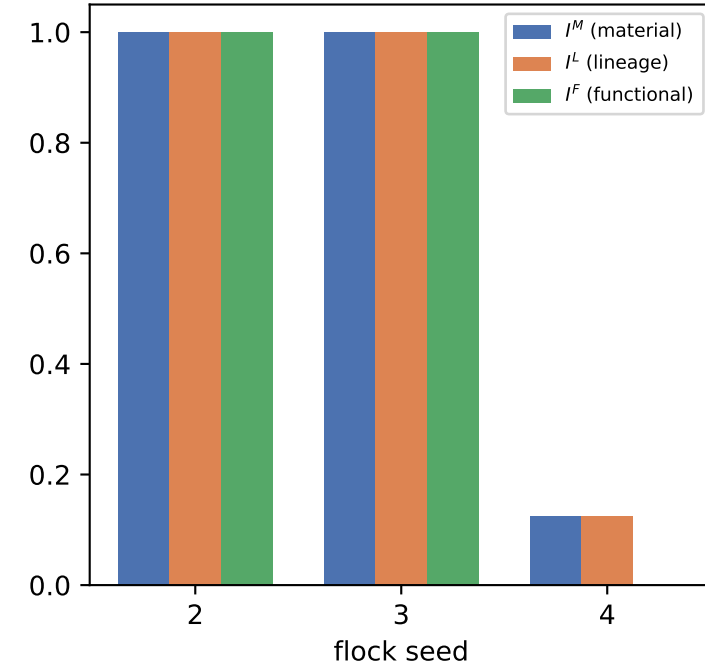
P(success)
