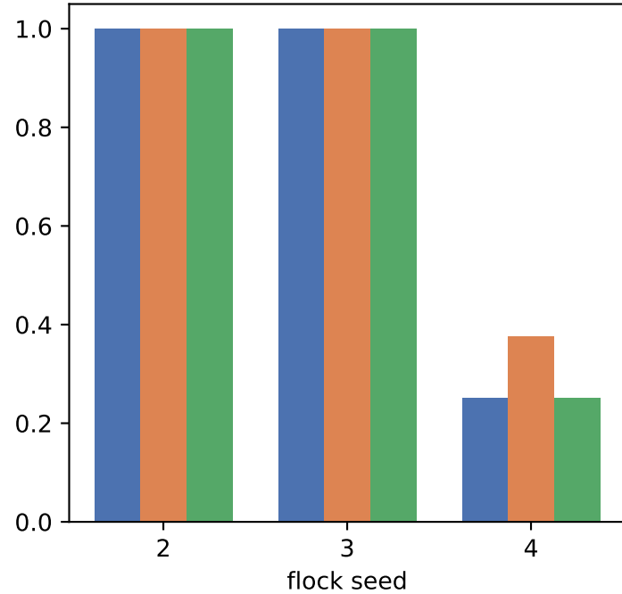
P(persistence)
