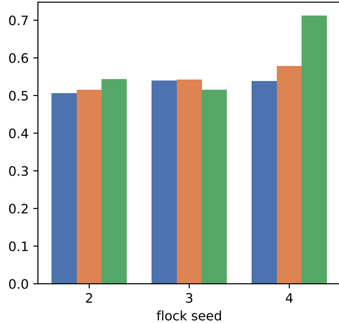
mean min coherence
