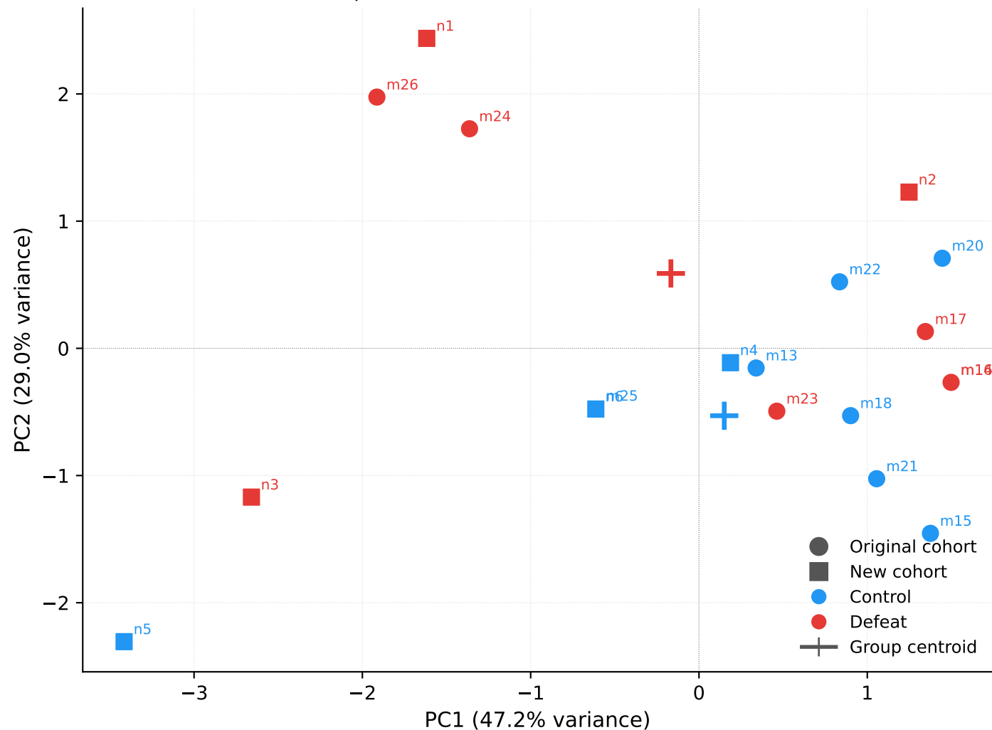
PCA — def3 parameters, combined cohort (n=19) [corrected]
