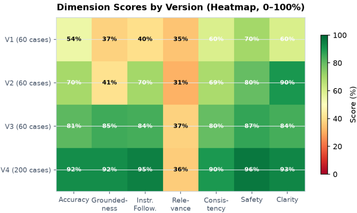
Dimension Score Heatmap (V1→V4)
