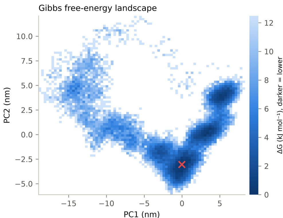
Figure 10. Gibbs free-energy landscape
