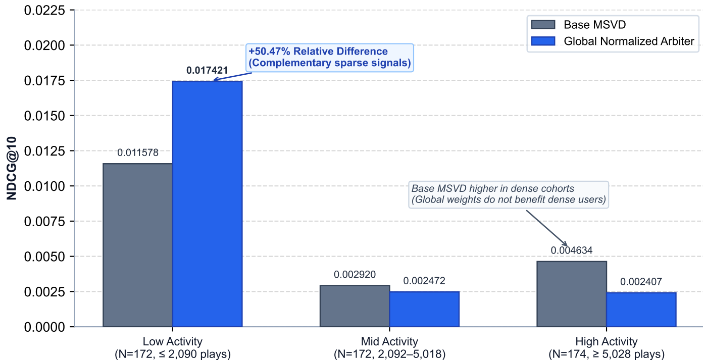
NDCG@10 by User Activity Segment
