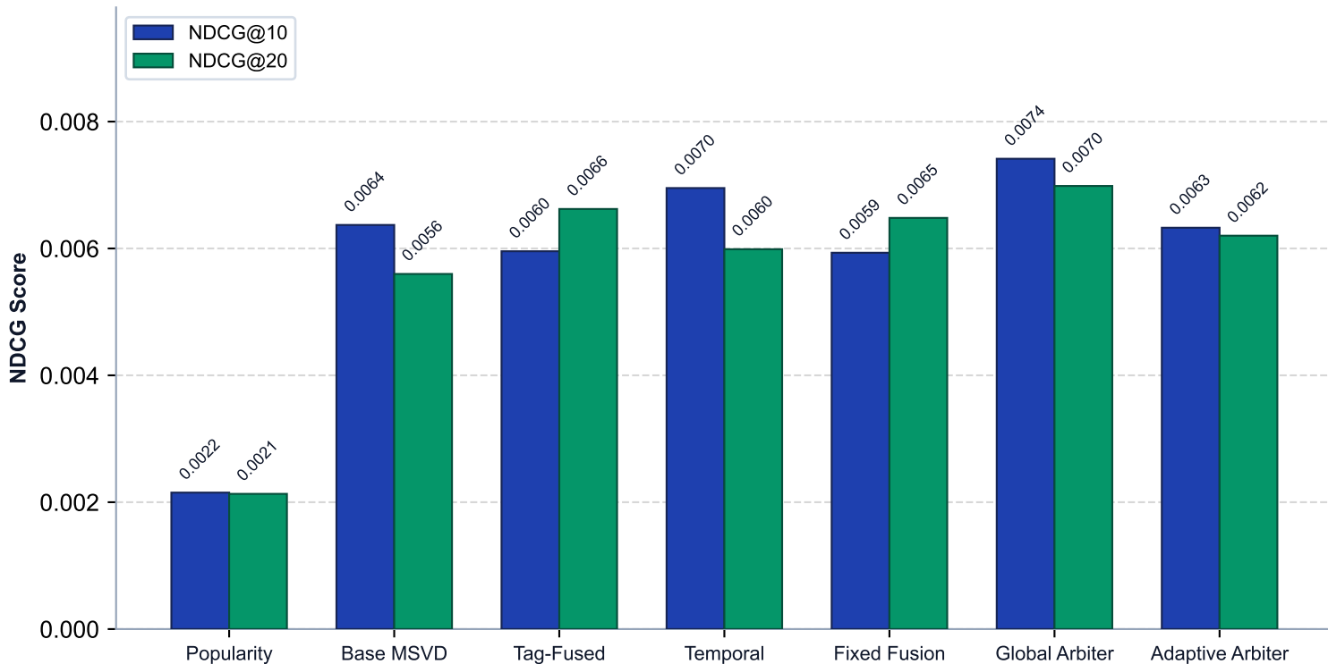
NDCG@10 and NDCG@20 Across Model Variants
