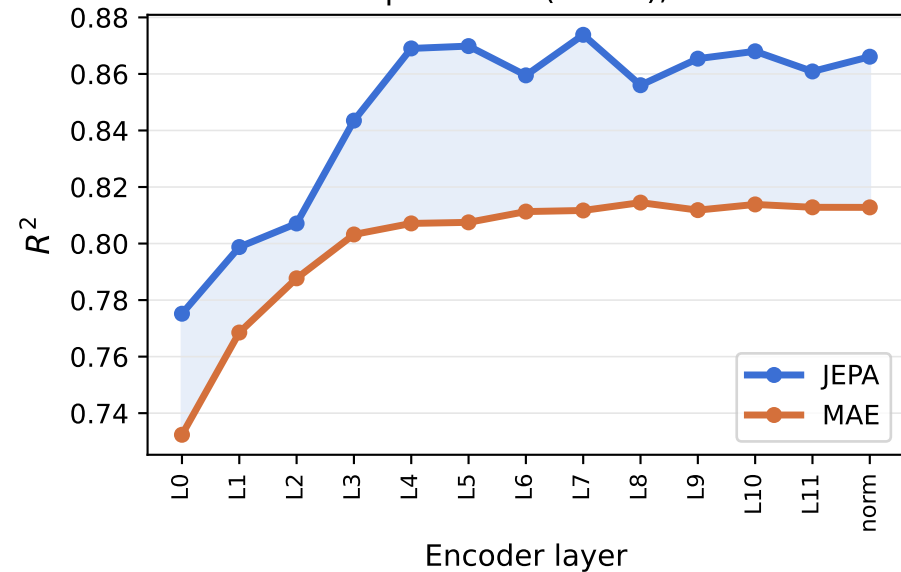
All 7 quantities (mean), t+32
