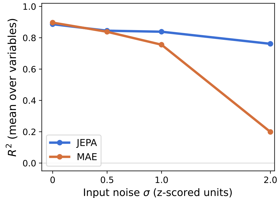
Active Matter
