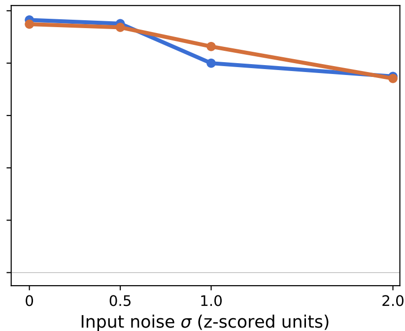
Shear Flow
