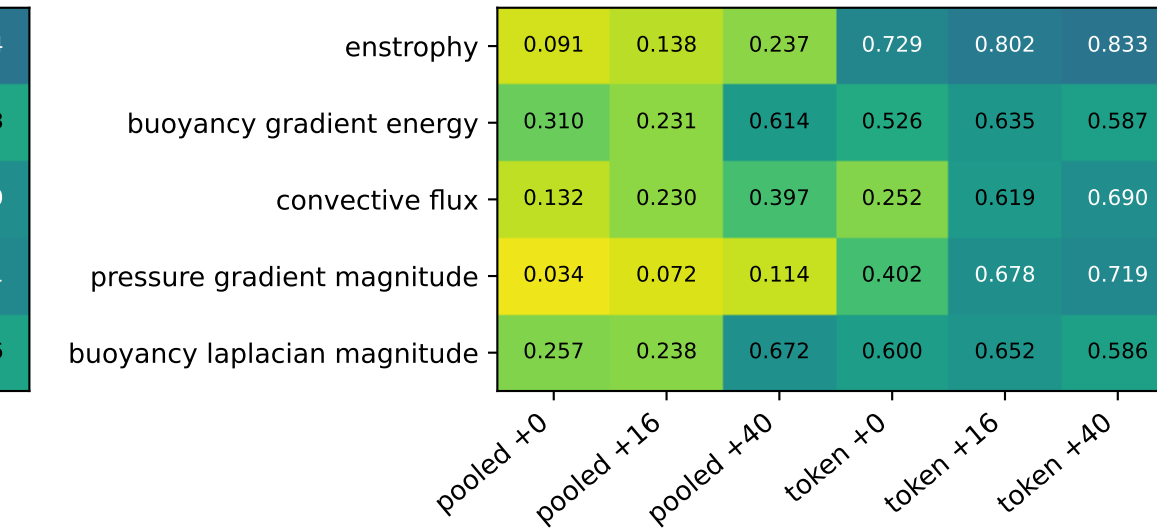
mae_future: ridge, test VRMSE
