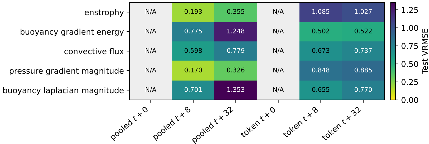
Persistence baseline, test VRMSE future prediction copies the corresponding current target
