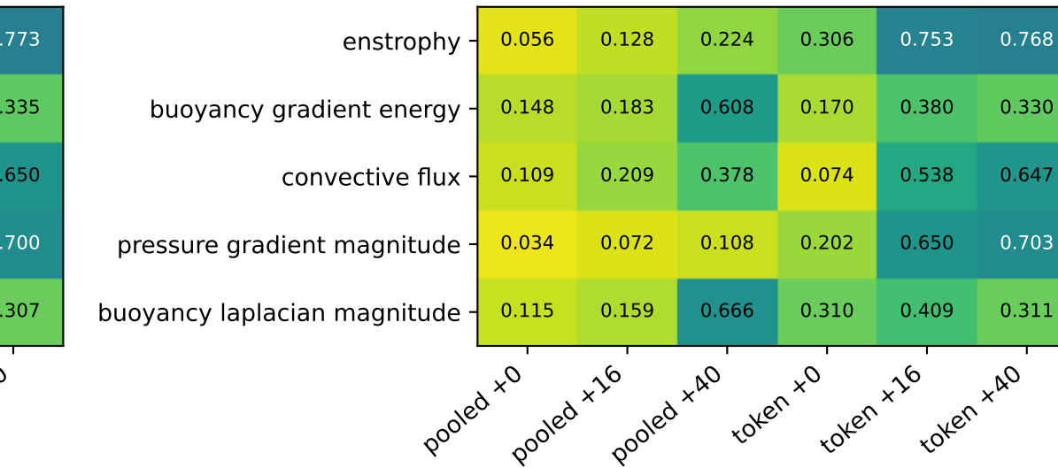
mae_future: selected, test VRMSE
