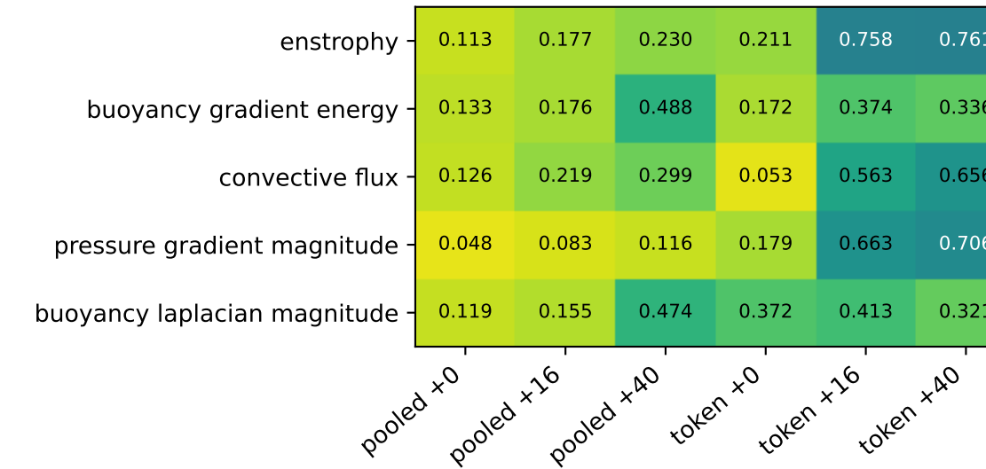
jepa: selected, test VRMSE
