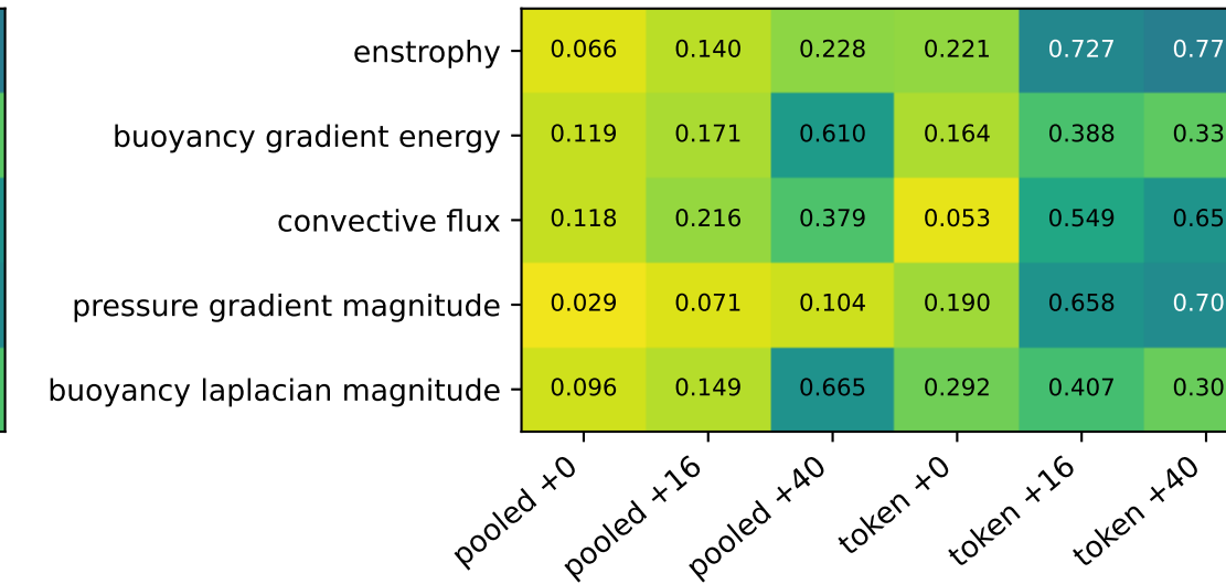
mae: selected, test VRMSE
