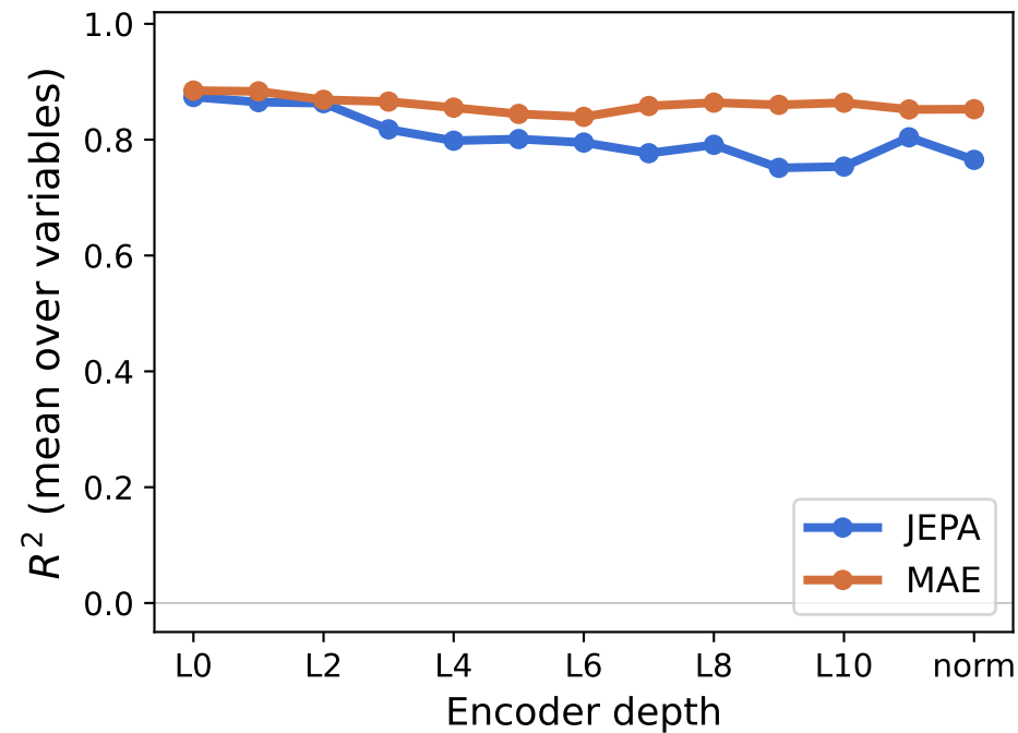
Active Matter
