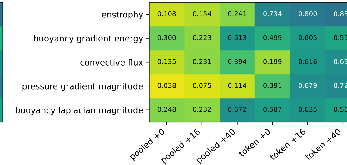
mae: ridge, test VRMSE
