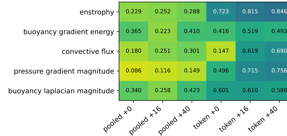
jepa_future: ridge, test VRMSE
