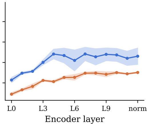
Velocity-buoyancy coh.
