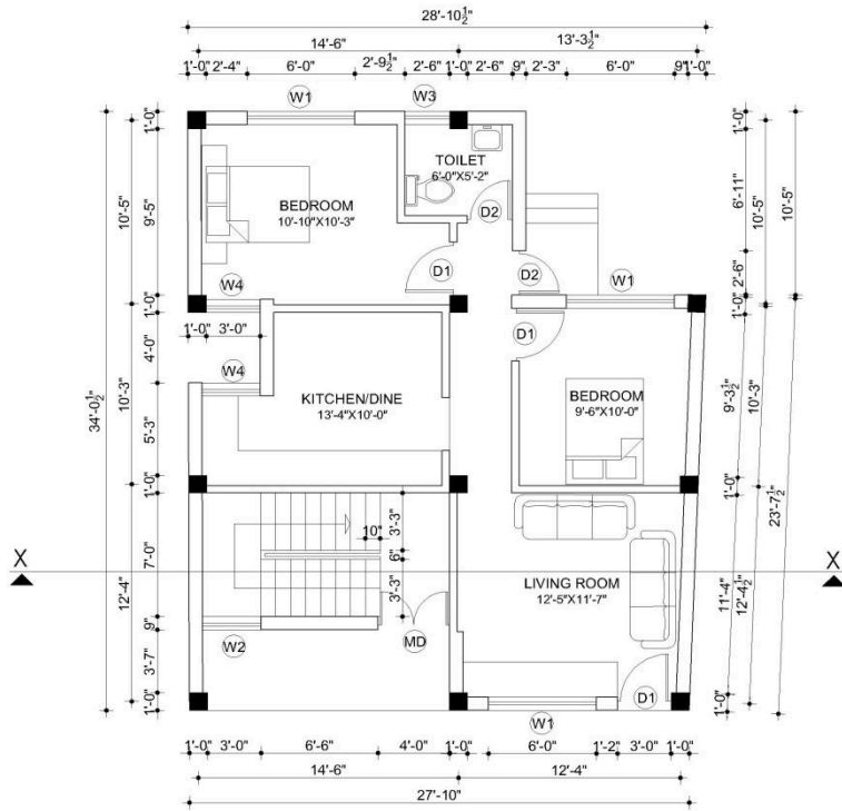
GROUND FLOOR PLAN 870.60 sq. ft.
