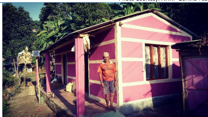
Caption: Gopal Damai's brick masonry cement mortar house with RCC band in Ajirkot rural municipality, ward no. 5, Mucchowk. The house owner was supported (financial and technical) by INF and he has received all the tranches.
