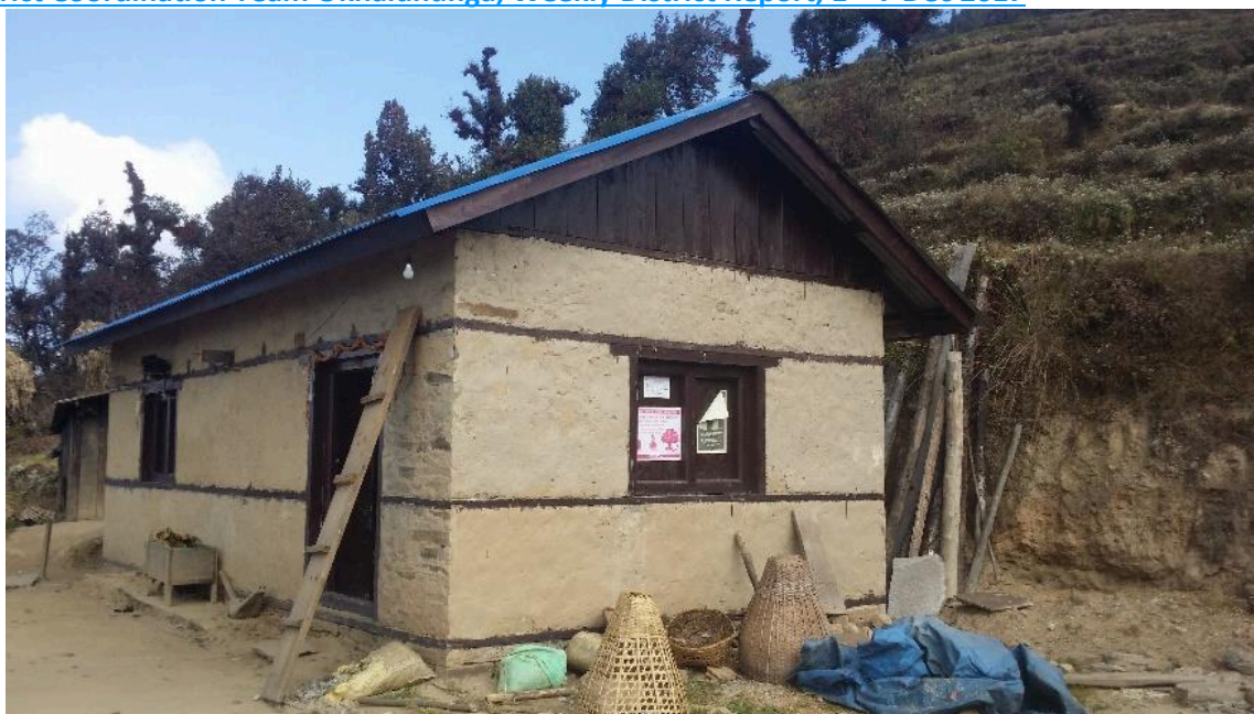
Baruneshwar VDC: single storey, stone and mud mortar masonry house, with timber bands. The home owner has received all three tranches.
