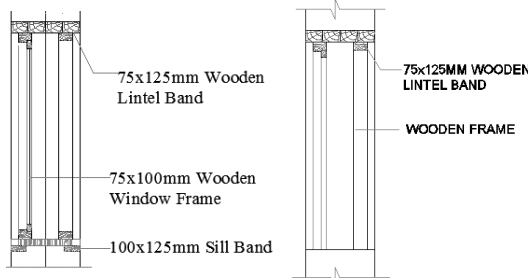
Window Section
