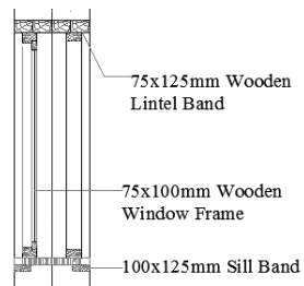
Window Section
