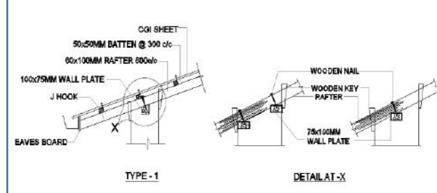
Detail of Rafter Joint with Wall Plate
