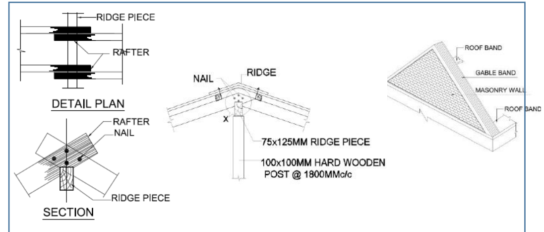
Detail of Rafter Joint at Ridge
