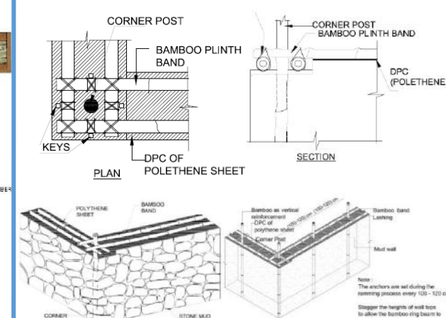
Bamboo for Horizontal and Vertical Band
