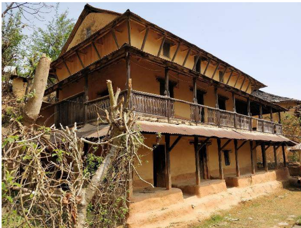
Waling Municipality, Jagat Bhanjyang, Ward No. 5, Syangja: this stone and mud mortar masonry house has survived three earthquakes; one in 1990 B.S., one in 2045 B.S., and one in 2072 B.S. The house is still standing despite the earthquakes and being more than 80 years old. The construction quality is quite good with support from timber bands at floor and roof level i.e. 2 bandings per floor.
