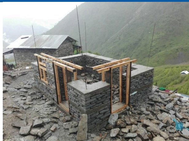
Caption: M/s. Masina Sunar's one room stone masonry mud mortar with RCC band house in Dharche rural municipality ward no 6, Kashigaon. The house owner has received second tranche.
