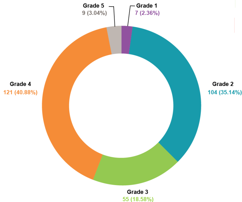
Damage Grade of House in Risk Area
