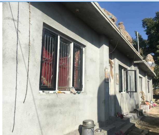
Pokharel gaun, Ward no 4, Changunarayan municipality one storey load bearing structure. Beneficiary have requested for the third tranche.
